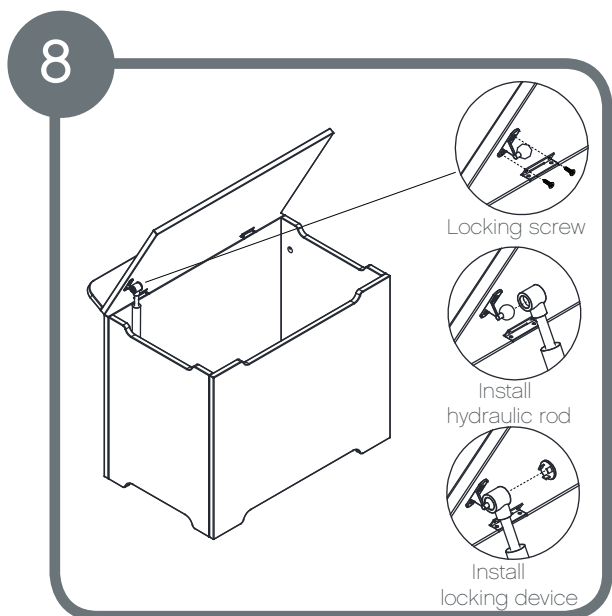
Assemble hydraulic rod
