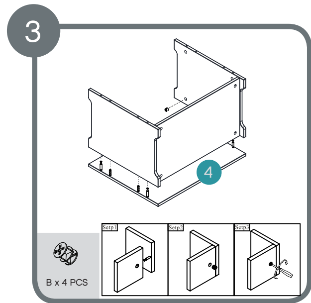
Assemble locking nuts 4 x B.
